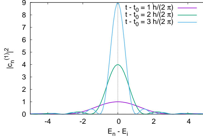
Figure 6.1: Transition probability |c_n^1(t)|^2 depending on E_n - E_i for various times t - t_0 , see (6.52).
