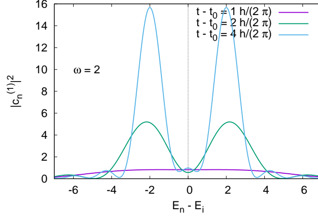
Figure 6.2: Transition probability |c_n^1(t)|^2 from (6.54) for \omega = 2 , depending on E_n - E_I and for various times t - t_0 .
