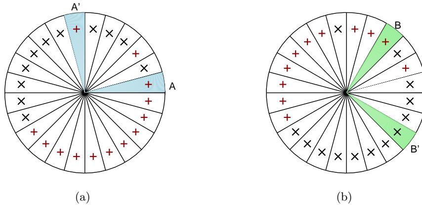
Figure 5.1: Advent-calendar like boxes for Alice and Bob, corresponding to the ‘hidden variable’ concept. Each drawer of each box contains a spin “up” or “down”, and Alice’s and Bob’s results are always opposite for drawers corresponding to any given direction. The shading shows directions that can be used to find a contradiction between quantum mechanics and these advent calendars, even if rules are introduced that allow only one drawer to be opened in each experiment.
